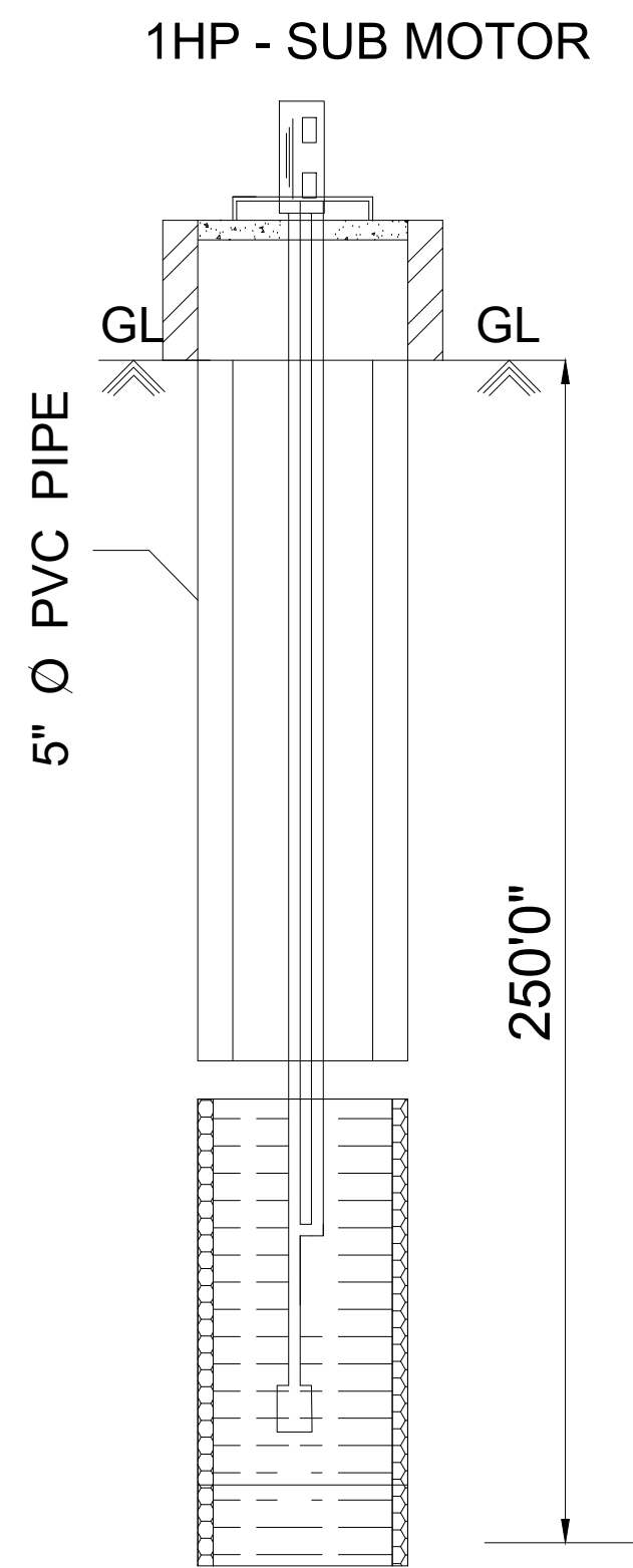
BOREWELL DETAILS
