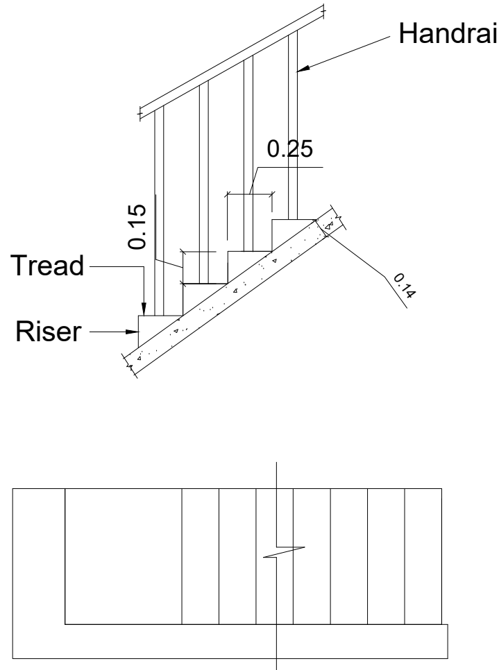
STAIRCASE DETAIL
