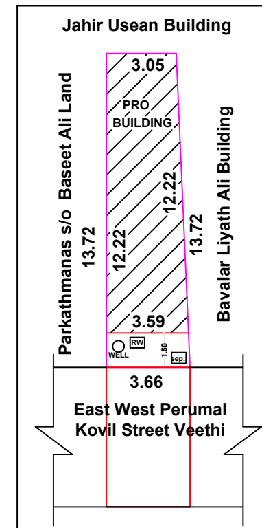
SITE PLAN & KEY PLAN
