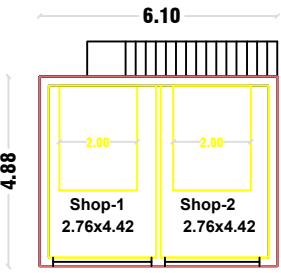
PRO. GROUND FLOOR PLAN
