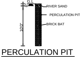
PERCOLATION PIT
