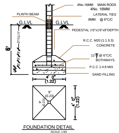
FOUNDATION DETAIL (SCALE: 1:50)
