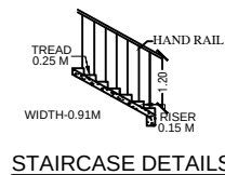
STAIRCASE DETAILS
