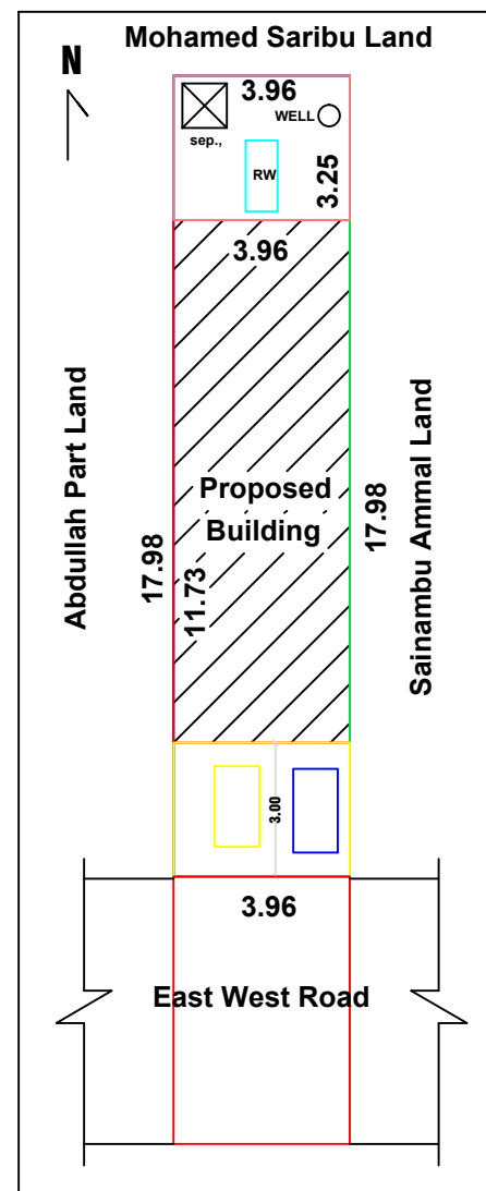
SITE PLAN CUM KEYPLAN
