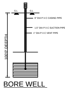
BORE WELL
