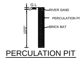
PERCULATION PIT
