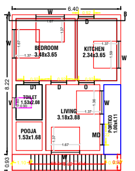
PRO., GROUND FLOOR PLAN
