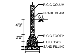
COLOUMN FOUNDATION
