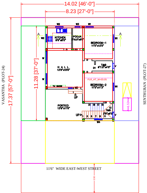
SITE CUM GROUND FLOOR
