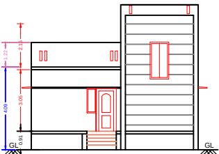
FRONT ELEVATION
