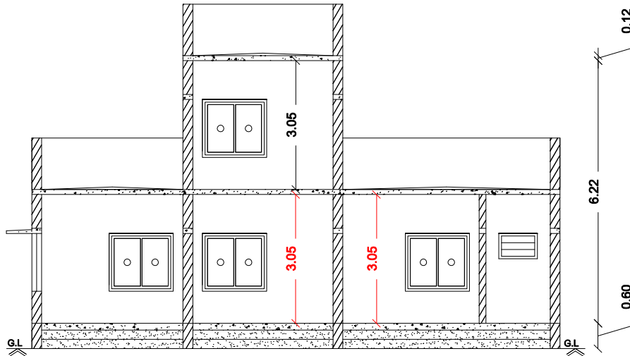
Section on-"AA"
