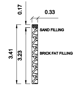
DETAILS OF PERCOLATION PIT
