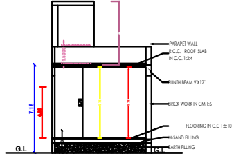
SECTION
