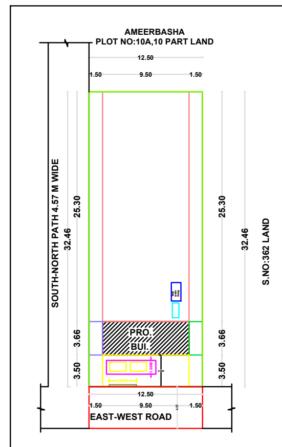
SITE PLAN & KEY PLAN
