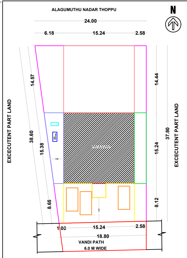
SITE PLAN & KEY PLAN
