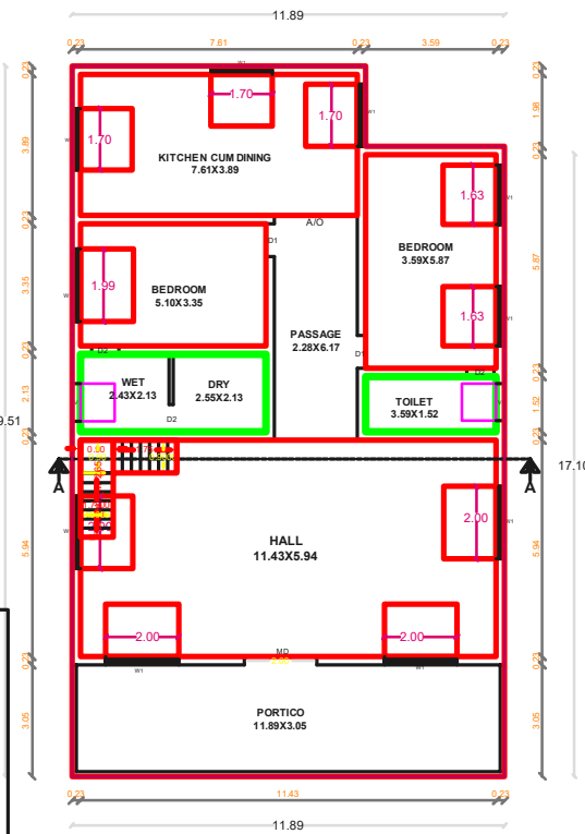
GROUND FLOOR PLAN PROPOSED
