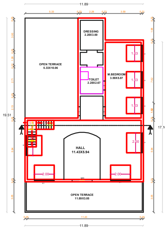
FIRST FLOOR PLAN PROPOSED
