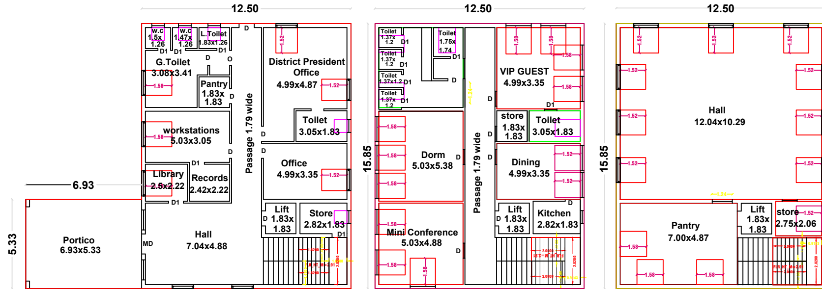
PROPOSED FIRST FLOOR PLAN PROPOSED SECOND FLOOR PLAN
