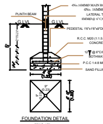
FOUNDATION DETAIL
