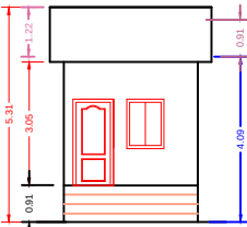
FRONT ELEVATION
