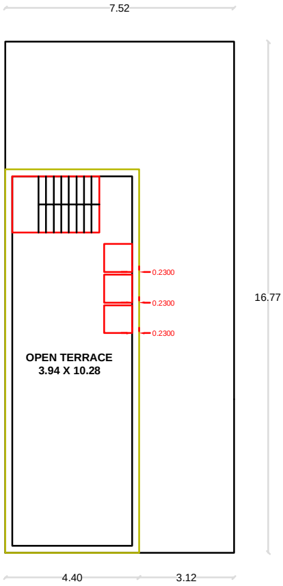
TERRACE FLOOR PLAN PROPOSED
