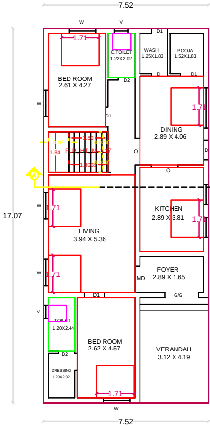
GROUND FLOOR PLAN PROPOSED
