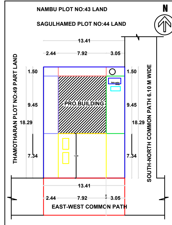
SITE PLAN & KEY PLAN
