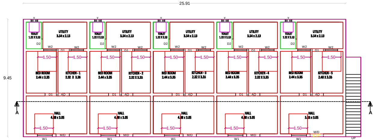
GROUND FLOOR PLAN PROPOSED
