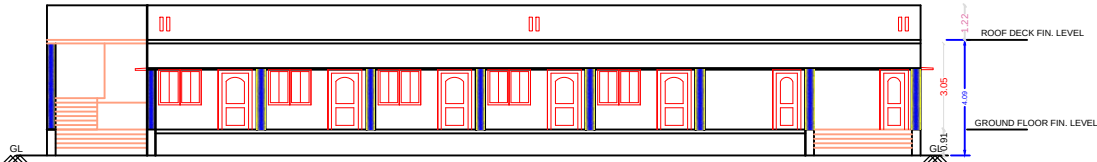
FRONT ELEVATION
