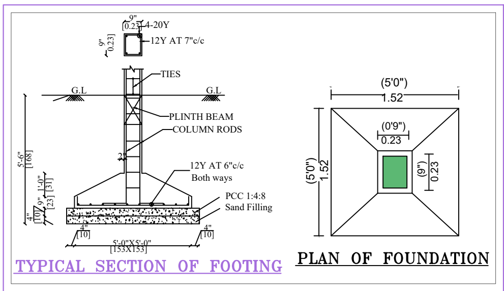
TYPICAL SECTION OF FOOTING
