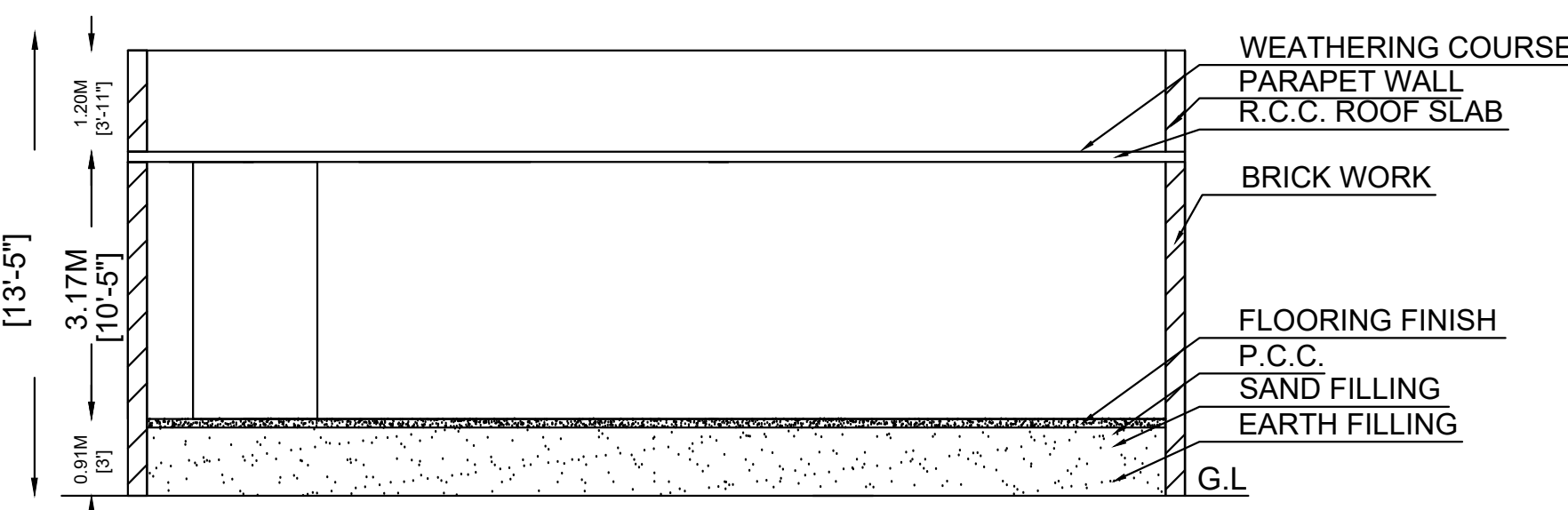
SECTION AN XX
