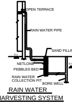
RAIN WATER HARVESTING SYSTEM
