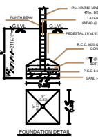
FOUNDATION DETAIL
