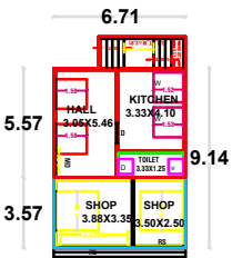
GROUND FLOOR PL
