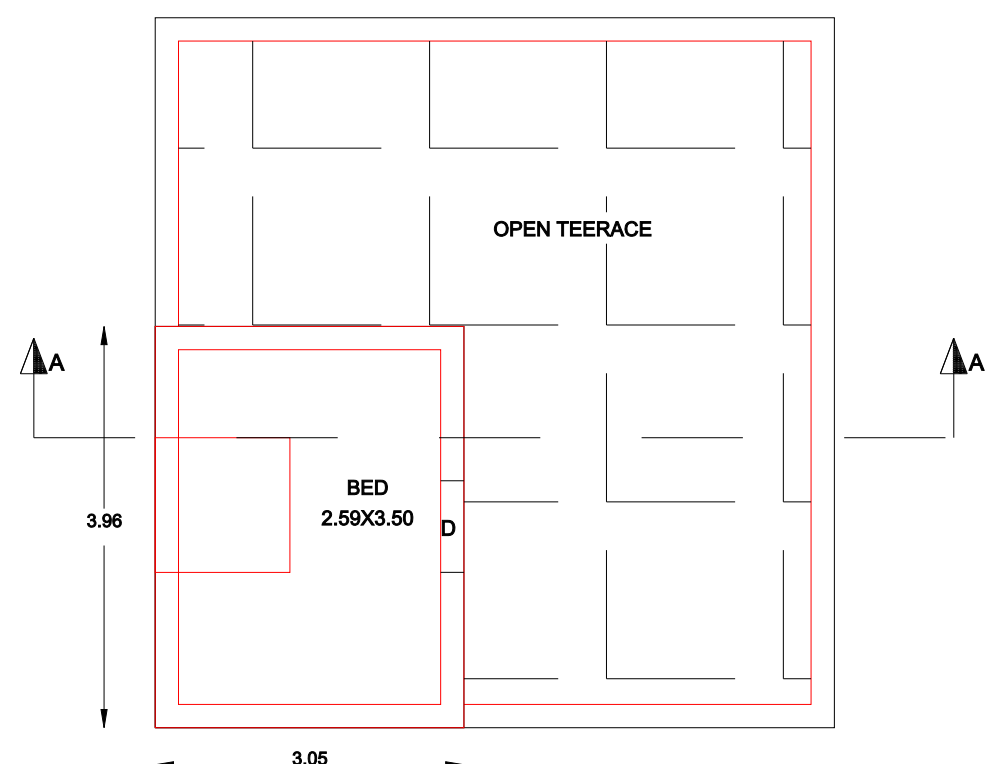
PROPOSED RESIDENTIAL FIRST FLOOR PLAN
