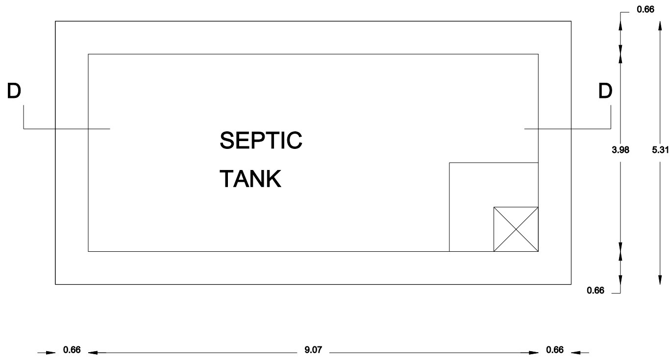
PLAN OF SEPTIC TANK SCALE 1"=2'0"
