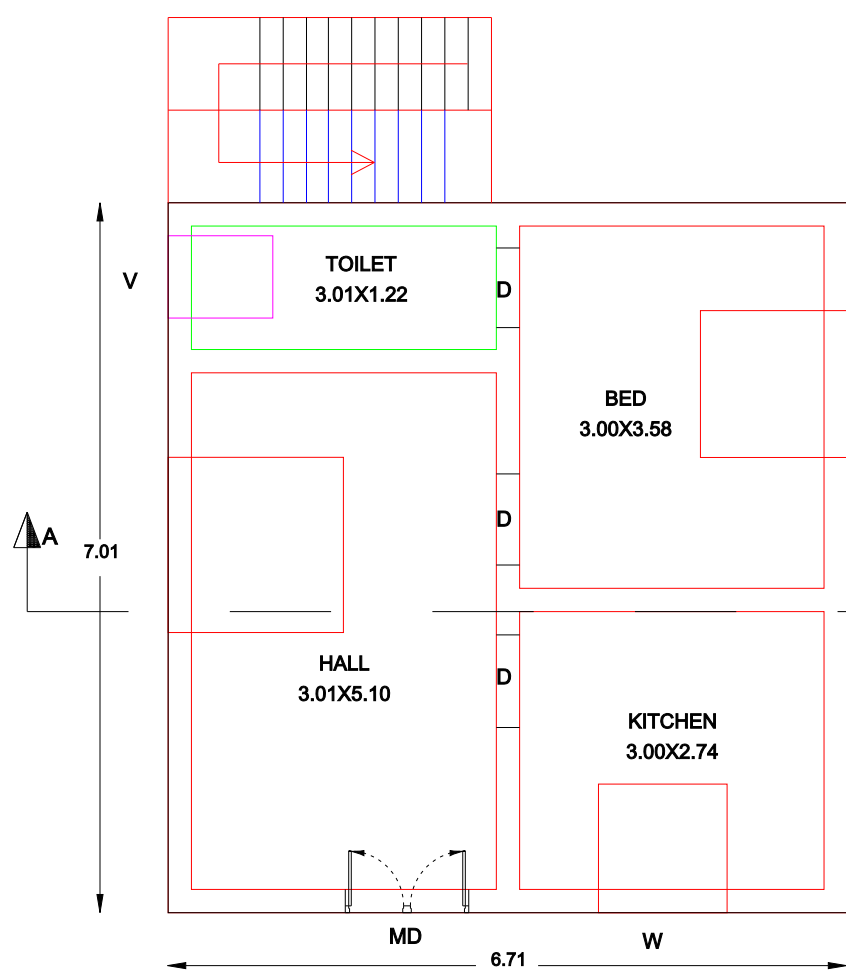
PROPOSED RESIDENTIAL GROUND FLOOR PLAN
