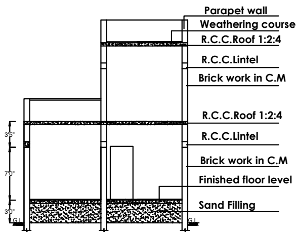
SECTION-'X-X'
