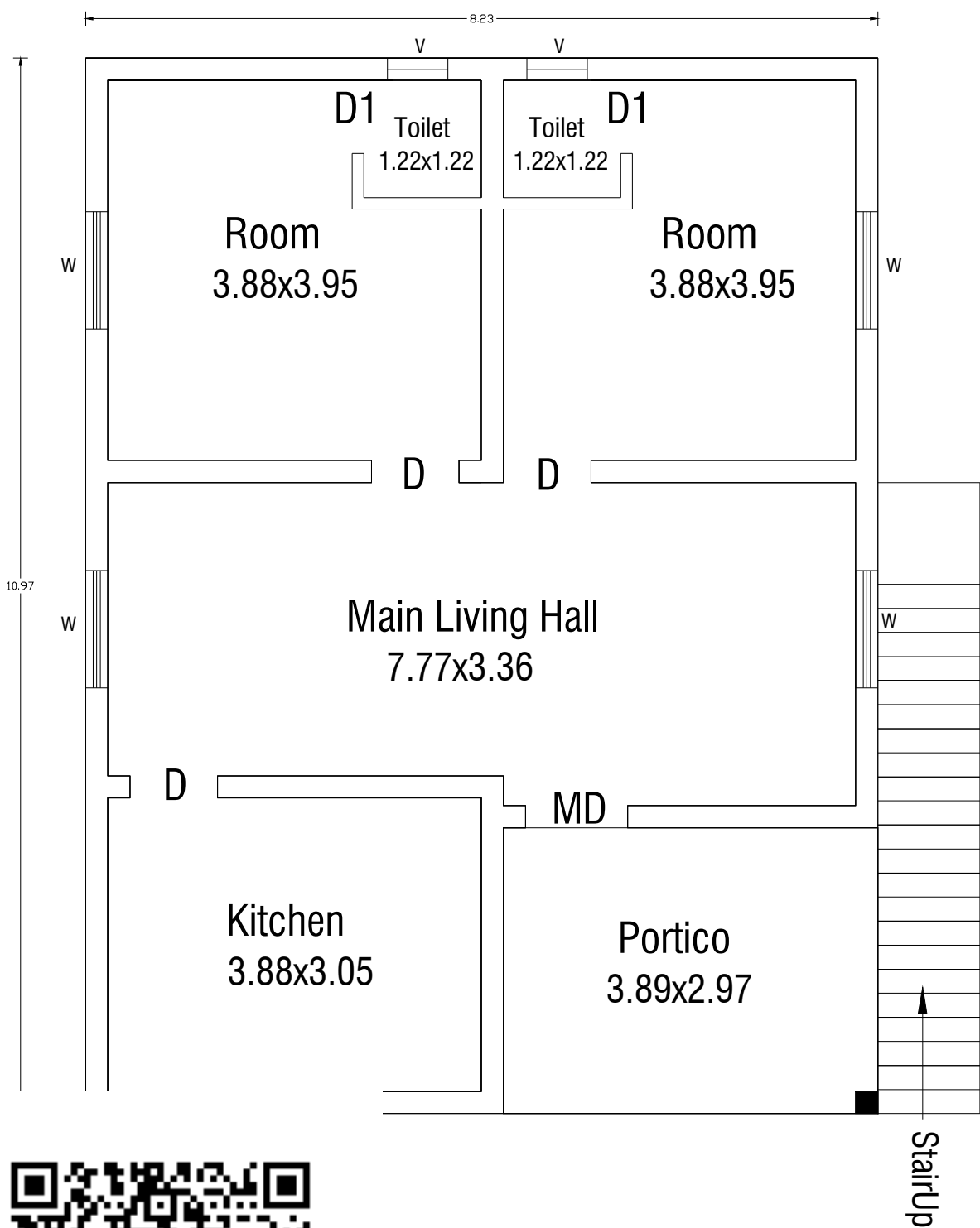
D GROUND FLOOR PLAN
