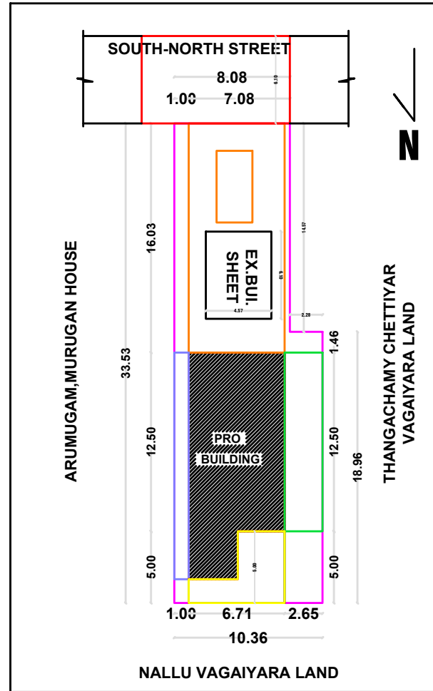
SITE PLAN & KEY PLAN
