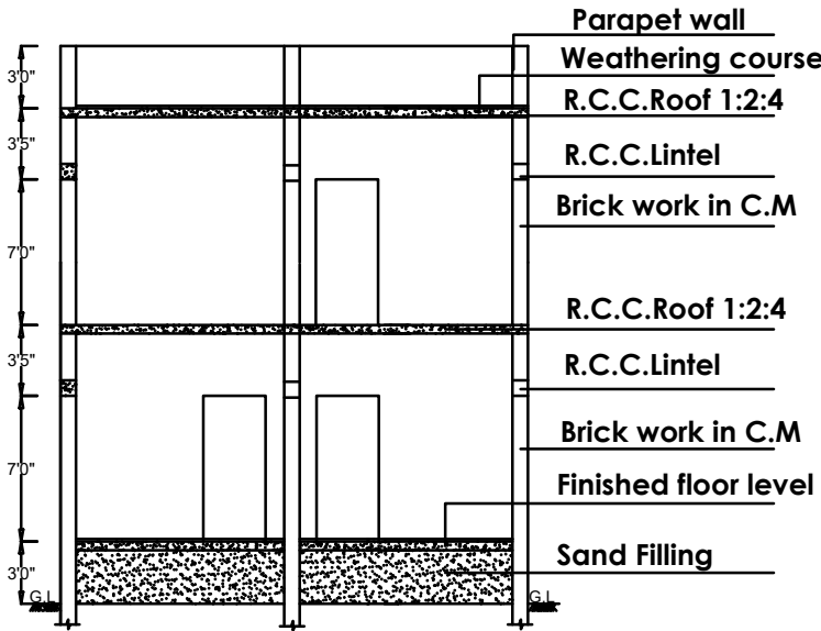
SECTION-'X-X'
