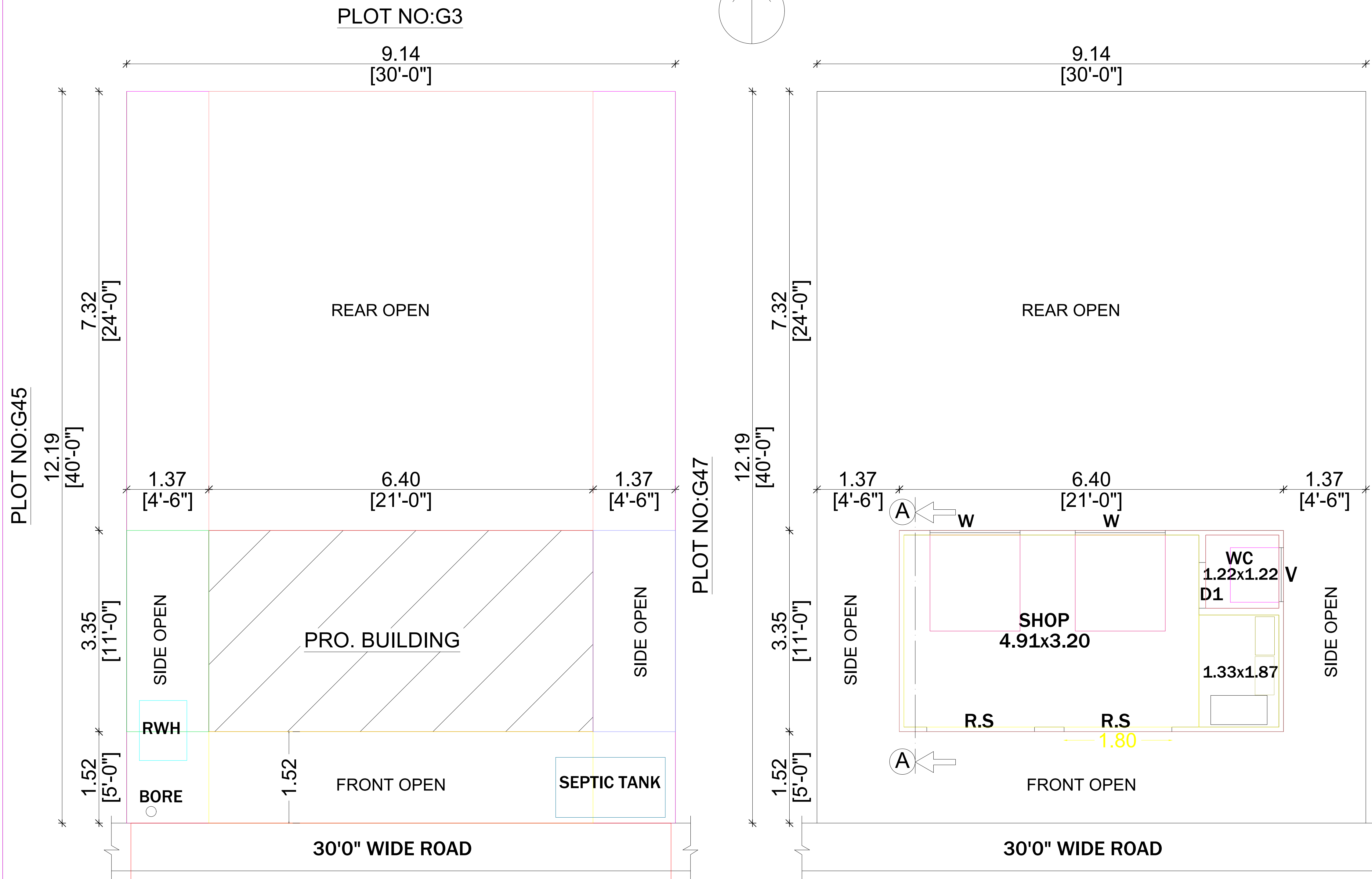
SITE PLAN
