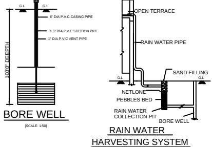
RAIN WATER HARVESTING SYSTEM
