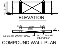
COMPOUND WALL PLAN
