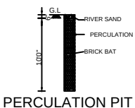
PERCOLATION PIT
