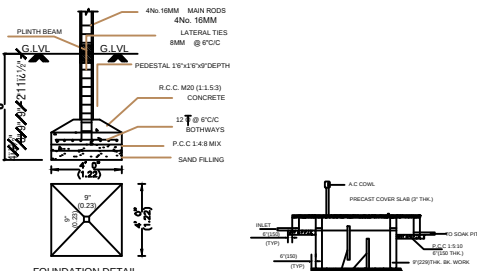
FOUNDATION DETAIL
