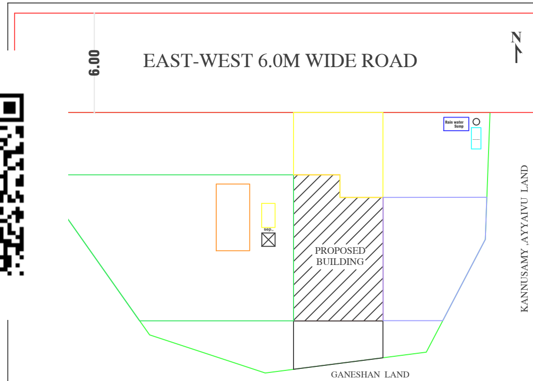
SITE PLAN CUM KEYPLAN
