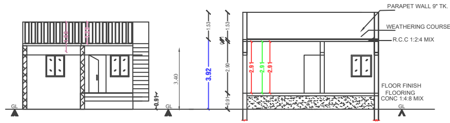
FRONT ELEVATION
