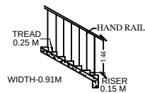
STAIRCASE DETAILS
