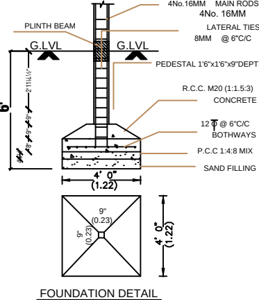
FOUNDATION DETAIL
