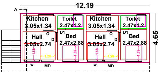
EXISTING GROUND FLOOR PLAN
