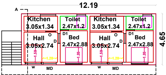
PROPOSED FIRST FLOOR PLAN
