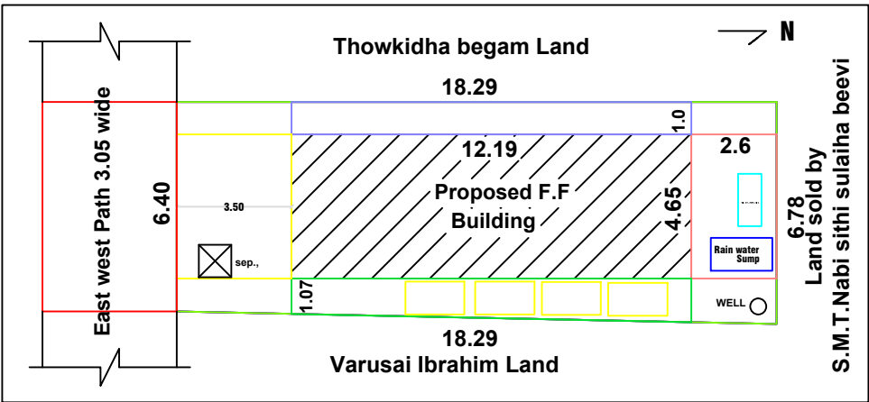
SITE PLAN CUM KEYPLAN
