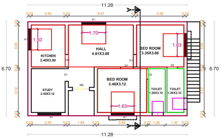
GROUND FLOOR PLAN PROPOSED
