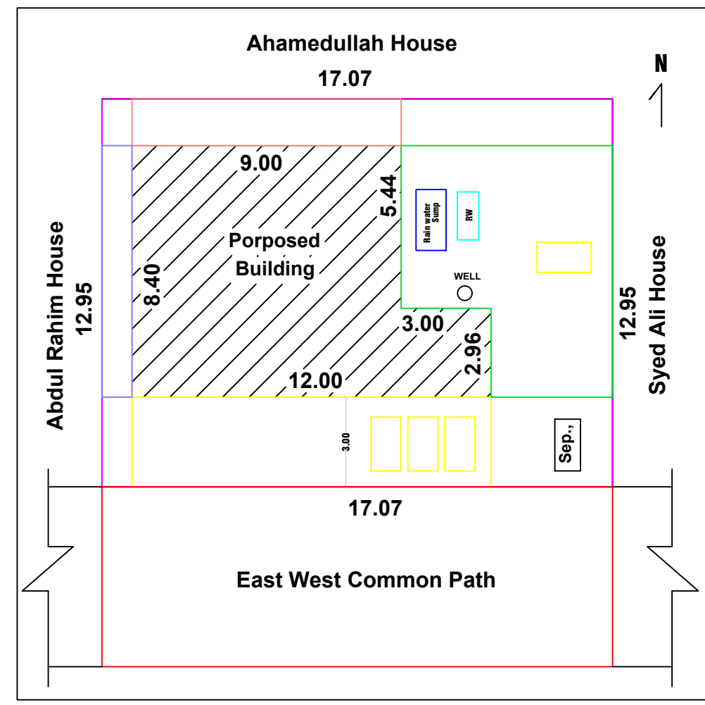
SITE PLAN CUM KEYPLAN
