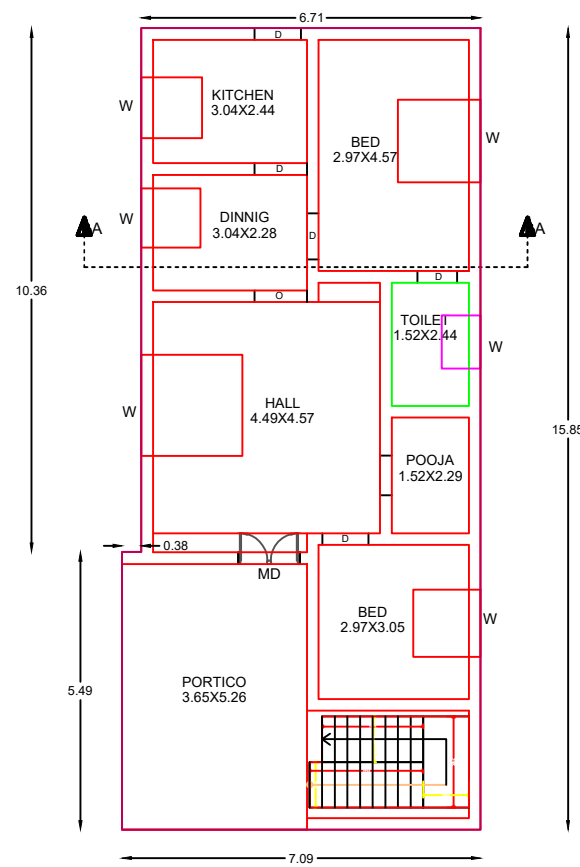
PROPOSED RESIDENTIAL GROUND FLOOR PLAN
