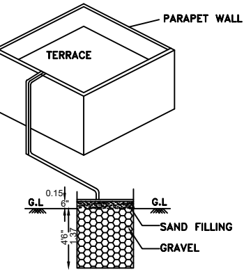
COLLECTION OF SUMP RAINWATER HARVESTING FROM TERRACE
