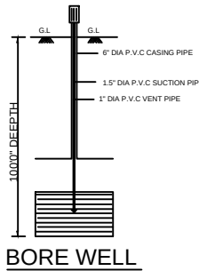
BORE WELL
