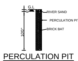
PERCOLATION PIT
