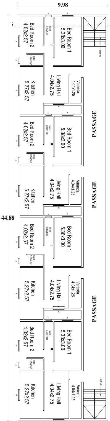
PROPOSED FIRST FLOOR PLAN
