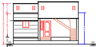
FRONT ELEVATION
