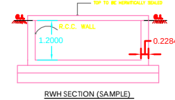
RWHP_CAPACITY_L=2000LTRS
