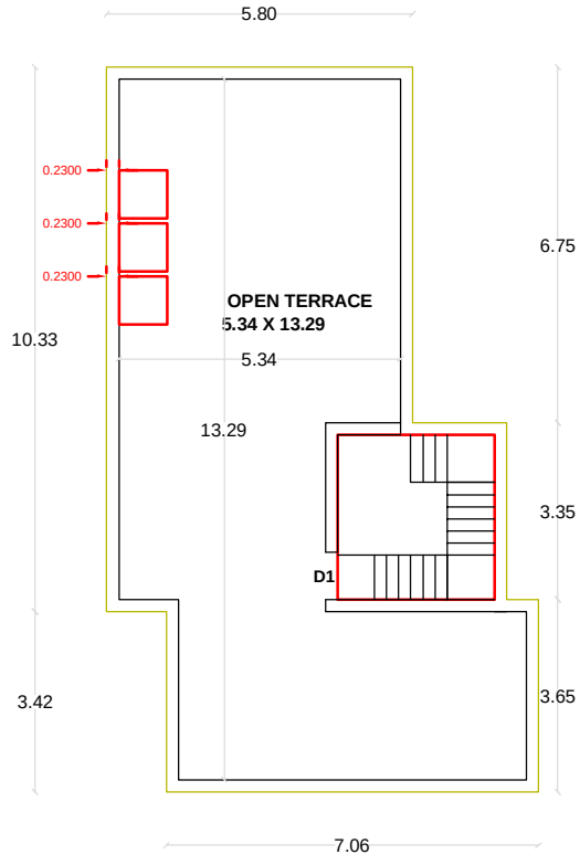
TERRACE FLOOR PLAN PROPOSED
