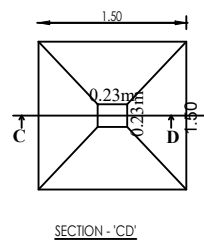
SECTION - 'CD'
