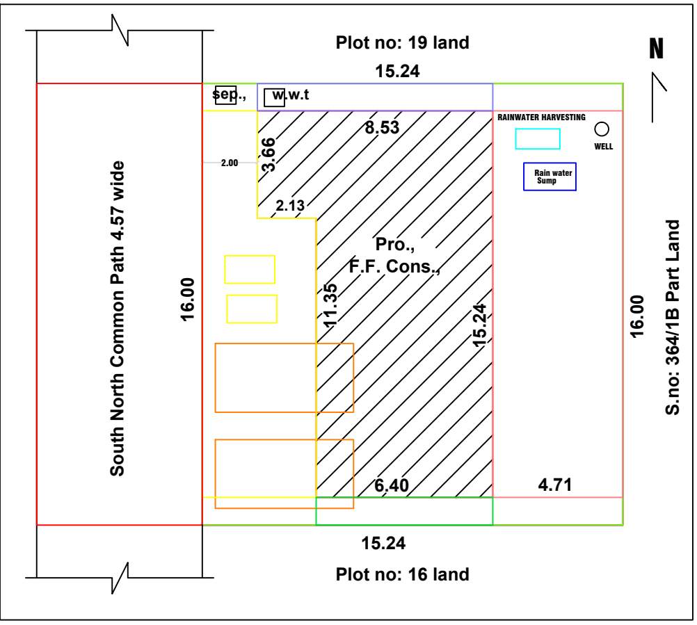
SITE PLAN CUM KEYPLAN
