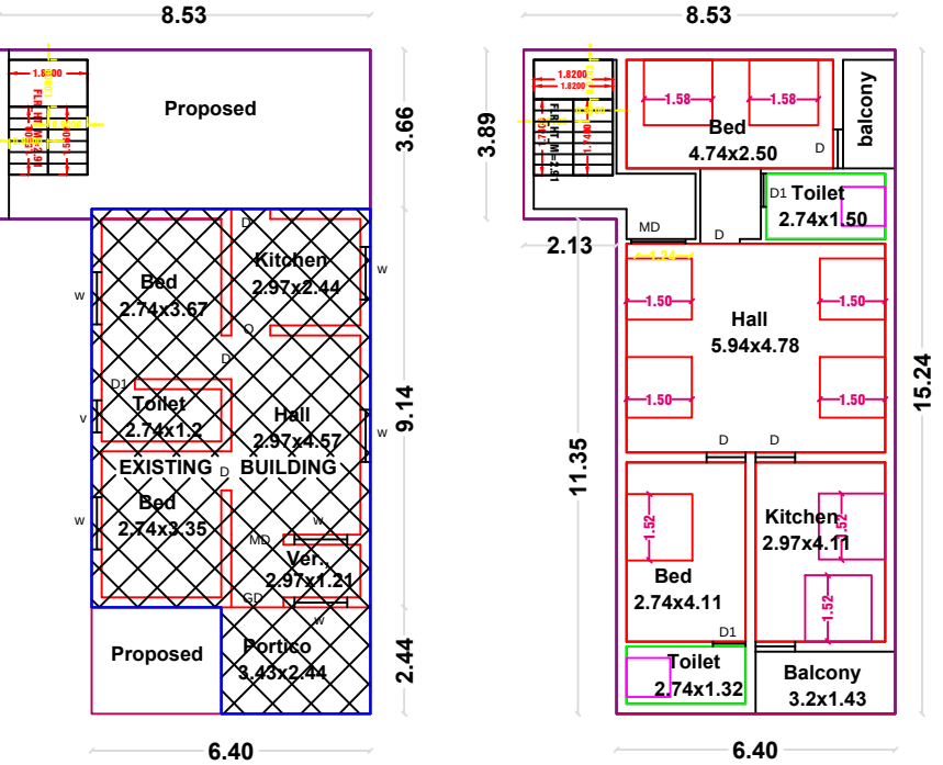
POSED FIRST FLOOR PLAN
