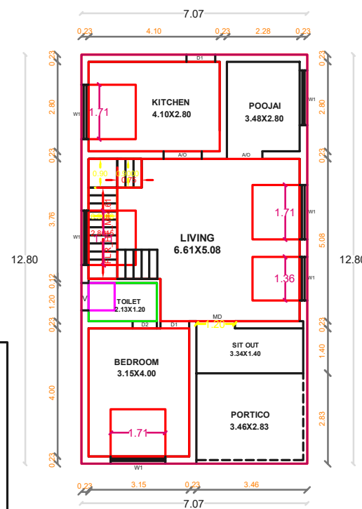
GROUND FLOOR PLAN PROPOSED
