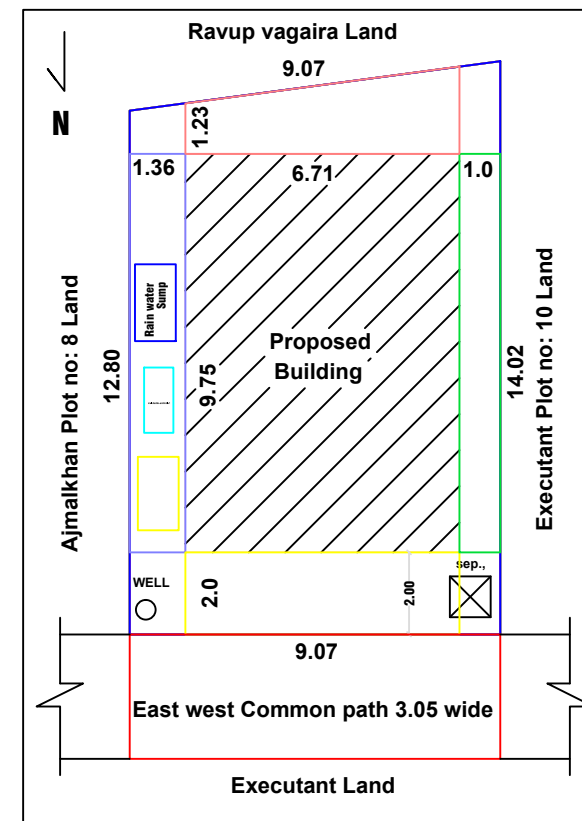
SITE PLAN CUM KEYPLAN
