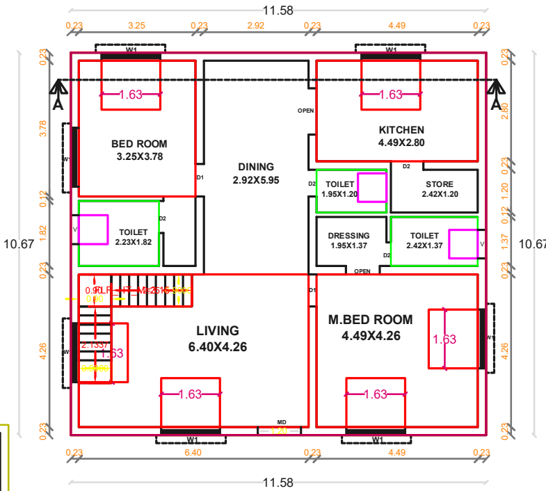
GROUND FLOOR PLAN PROPOSED
