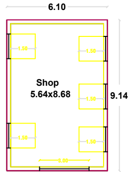
PRO. GROUND FLOOR PLAN
