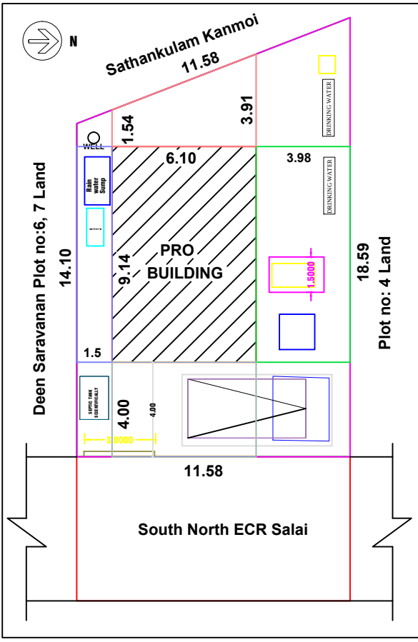
SITE PLAN & KEY PLAN
