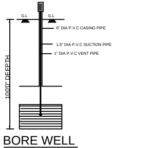
BORE WELL
