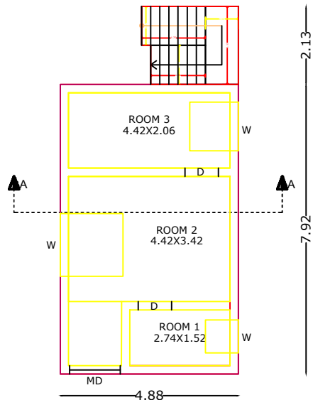
PROPOSED COMMERCIAL GROUND FLOOR PLAN
