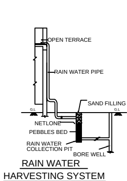
RAIN WATER HARVESTING SYSTEM
