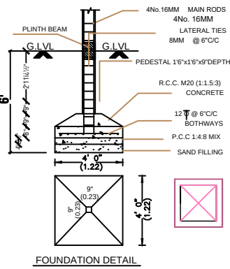
FOUNDATION DETAIL
