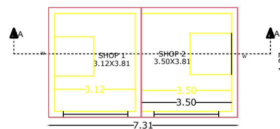
EXISTING COMMERCIAL GROUND FLOOR BUILDING & PROPOSED COMMERCIAL GROUND FLOOR PLAN
