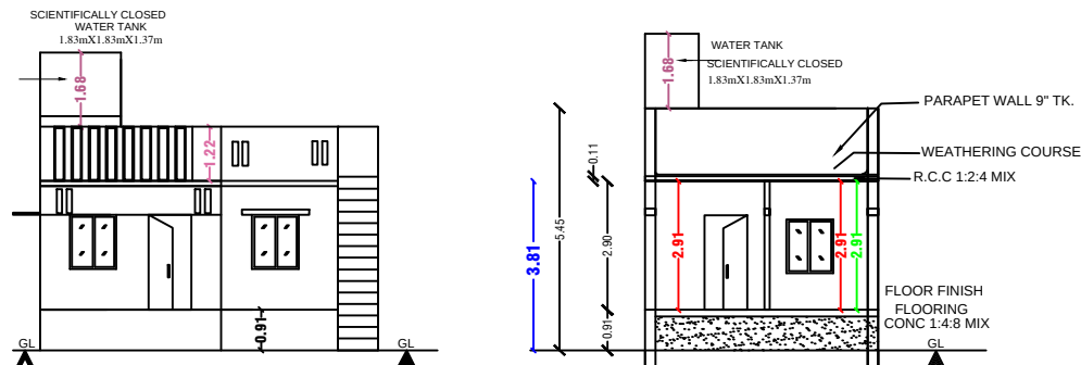
FRONT ELEVATION
