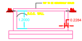
RWH SECTION (SAMPLE) RWH_CAPACITY_L=2000LTRS
