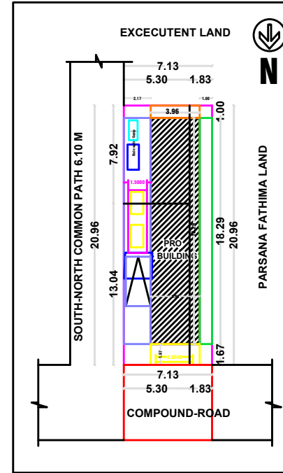
SITE PLAN & KEY PLAN
